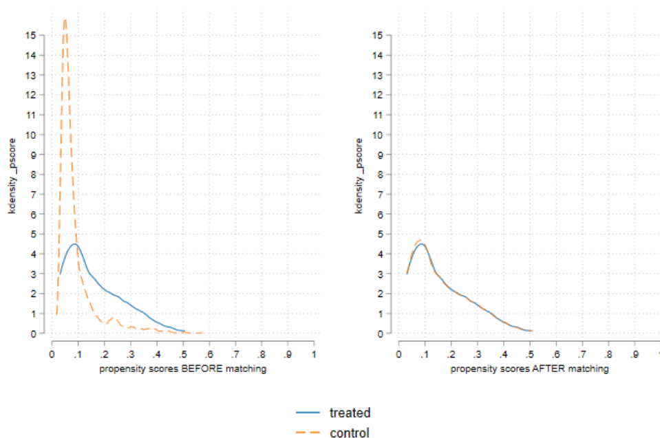
Figure A.1: Propensity score before and after matching
