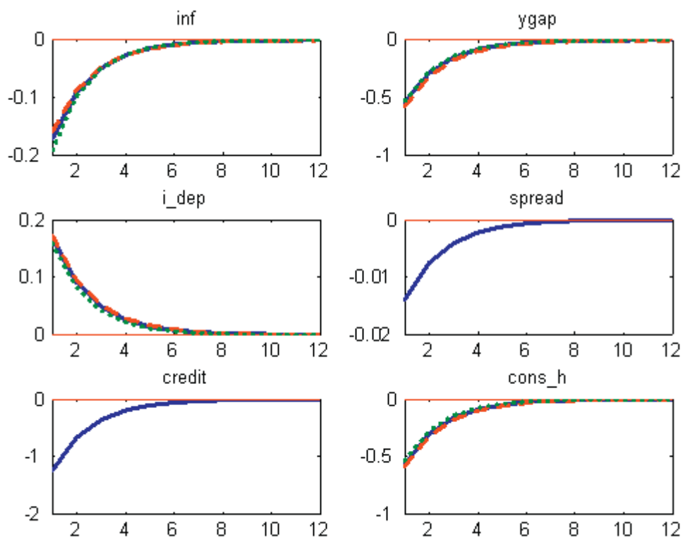
Figure 2: Impulse responses to a policy shock under a Taylor rule within different models
