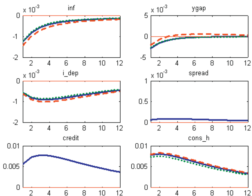
Figure 1: Impulse responses to a technology shock under a Taylor rule within different models
