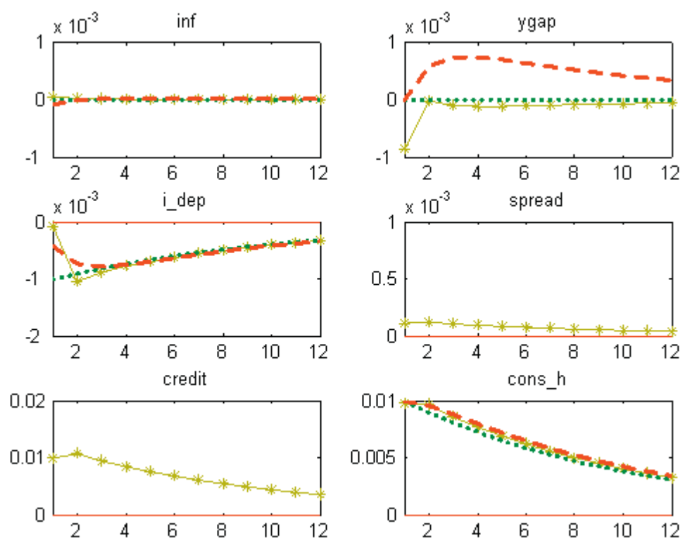
Figure 3: Impulse responses to a technology shock under optimal policy within different models
