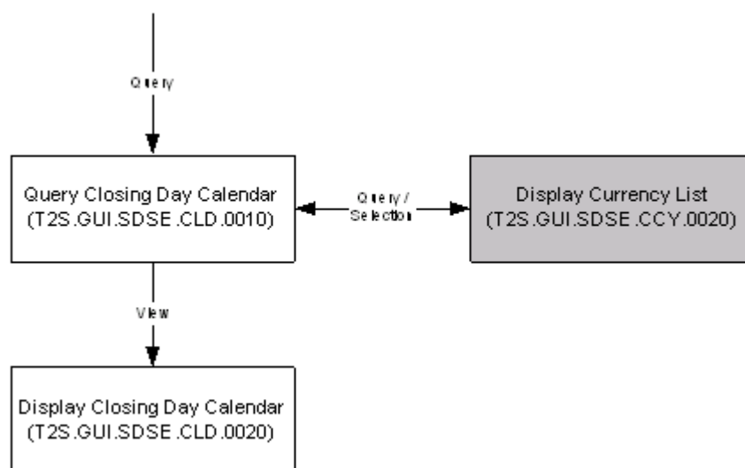
Figure 4-41 Closing Day Calendar Query and Maintenance user interface framework
