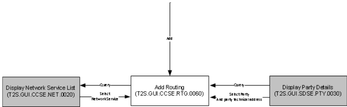
Figure 7-4 Add routing user interface framework
