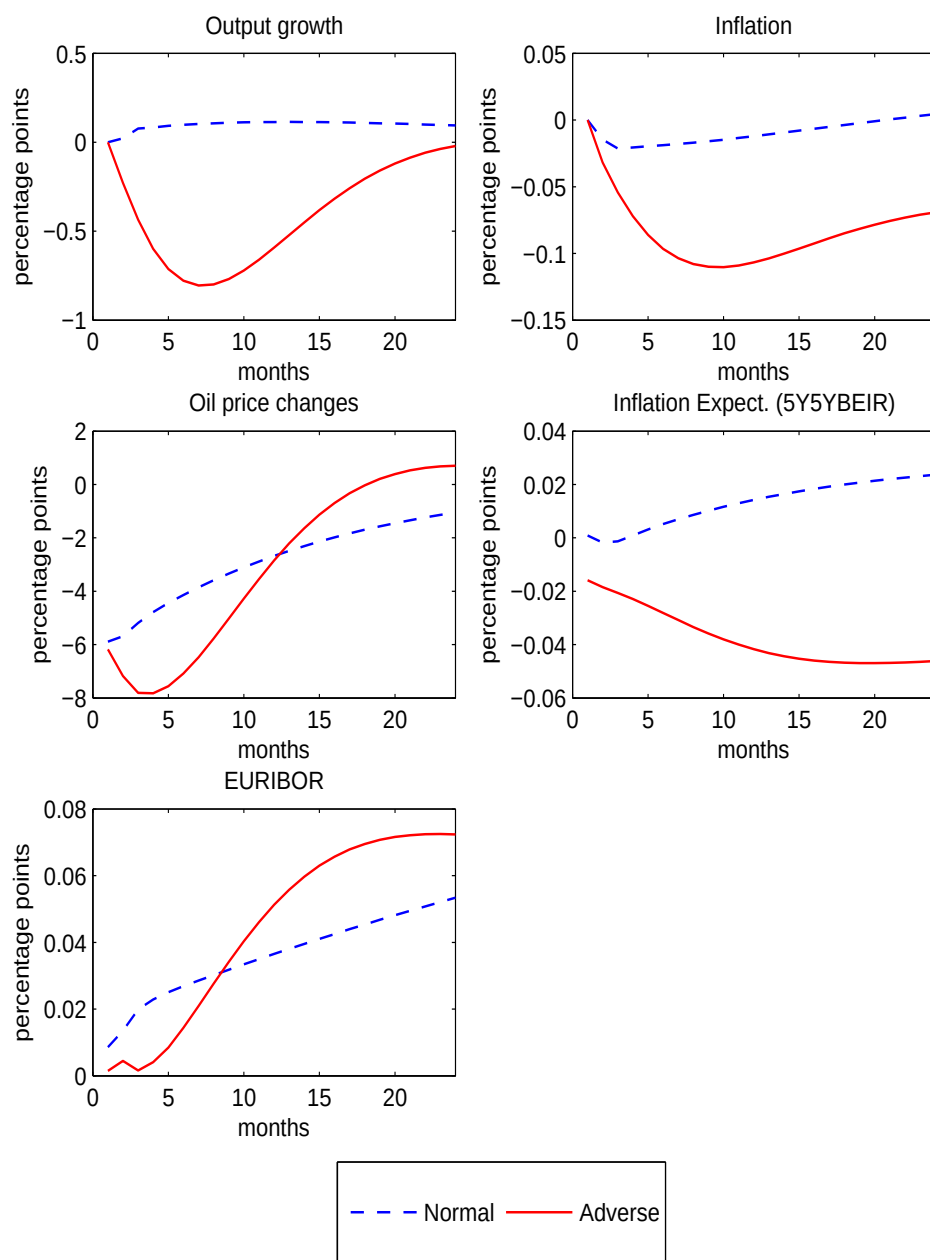
Figure 5: Impulse responses to oil price shock (one standard deviation shock), slashed blue: normal regime, solid red: adverse regime
