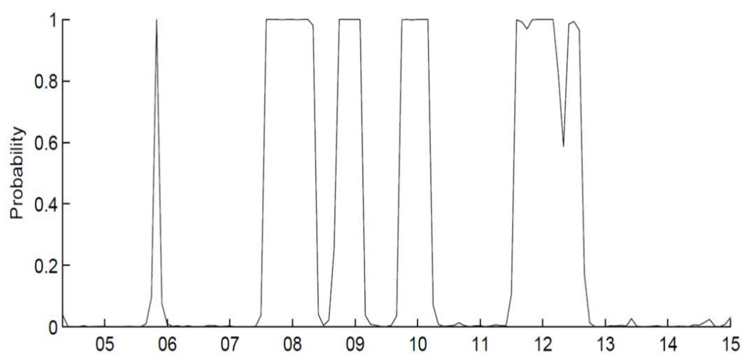
Figure 3: Probability of high-variance regime
