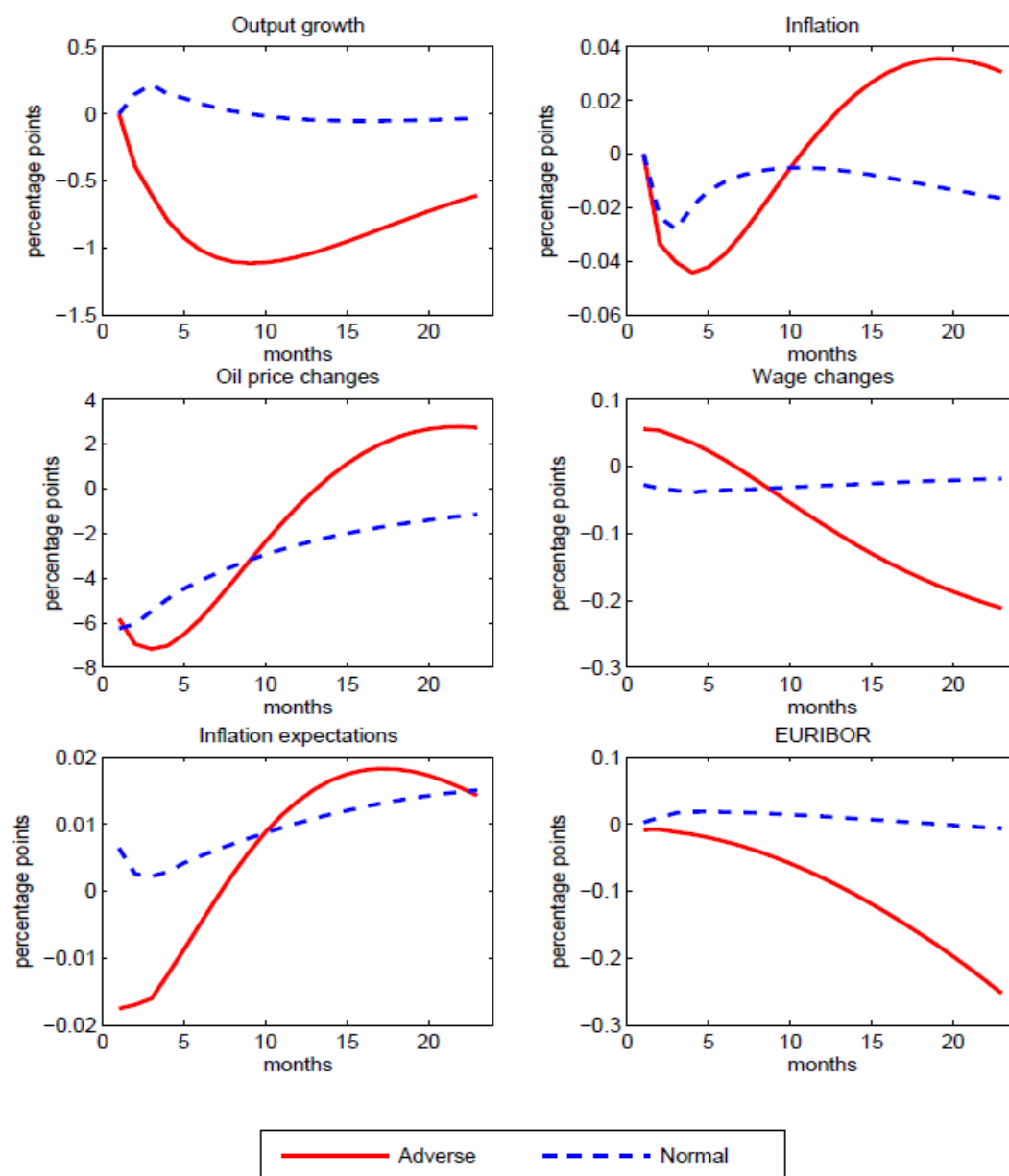
Figure 7: Impulse responses to oil price shock in model with nominal negotiated wages (one standard deviation shock), slashed blue: normal regime, solid red: adverse regime
