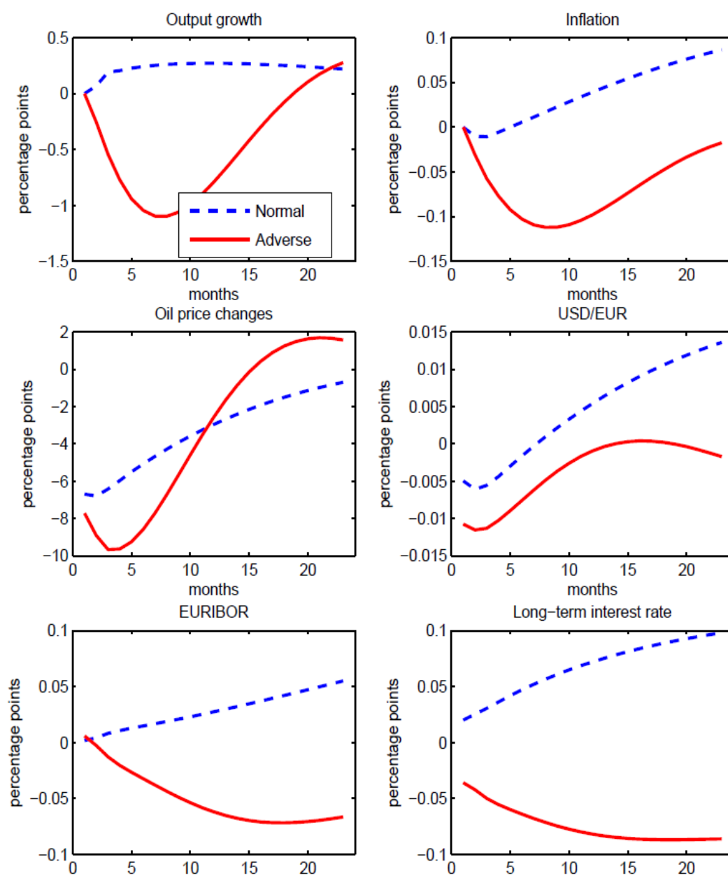
Figure 8: Impulse responses to oil price shock in model with long-term real interest rate (one standard deviation shock), slashed blue: normal regime, solid red: adverse regime
