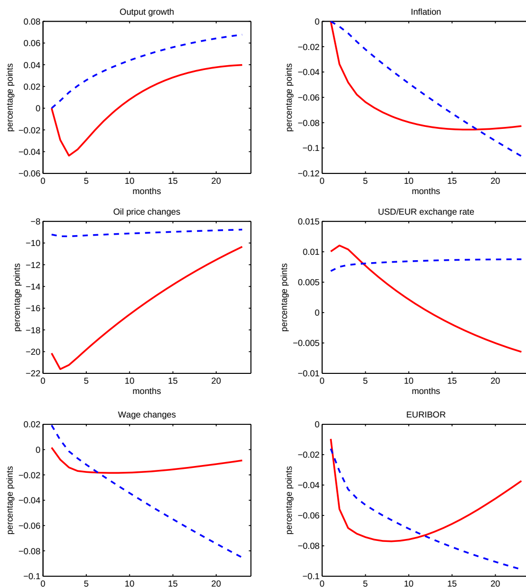
Figure 9: Impulse responses to oil price shock for 1974-2015 sample, slashed blue: normal regime, solid red: adverse regime
