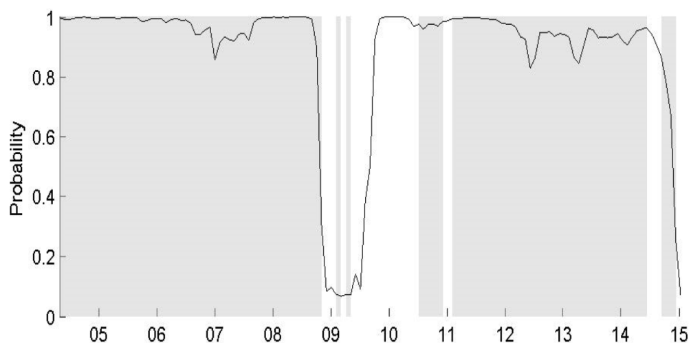
Figure 2: Time-varying probability for being in a normal regime (grey-shaded area) and conditional probability of staying in that regime (black line)
