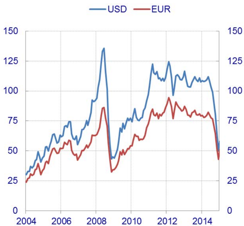
Figure 10: Evolution of Brent crude oil prices ( in different currencies )
