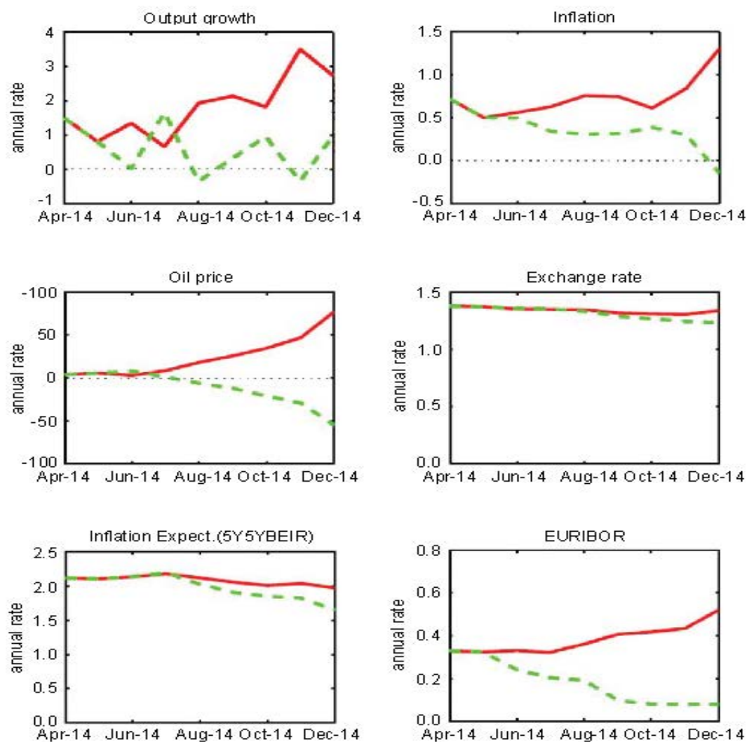
Figure 4: Counterfactual experiment: normal instead of adverse regime (green dashed line: actual data, red solid line: counterfactual path)
