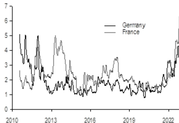
1M MA of yield RMSE for German and French par curves; bp 1
